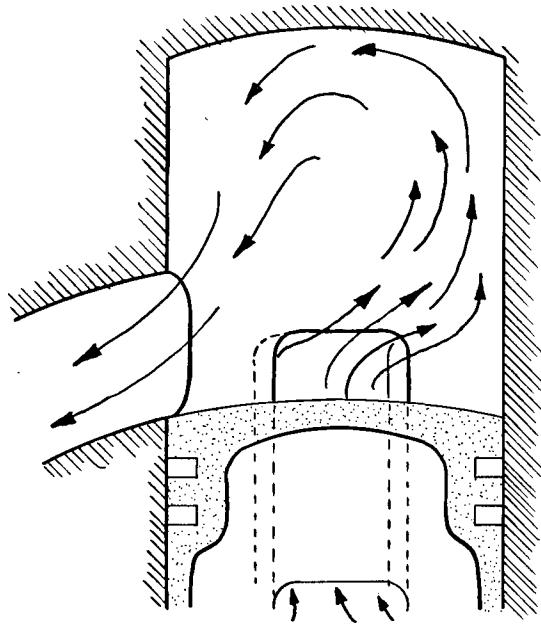
Dr. Schneurle's "loop" scavenging system and its variants have been almost universally adopted by makers of high output two-strokes.
